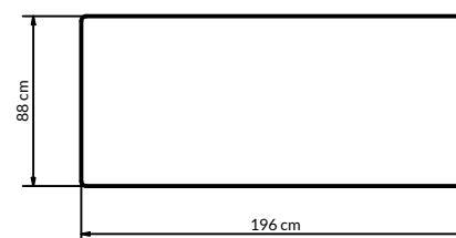
CLASSIC LINE - LARGE
